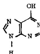
hypoxanthine
